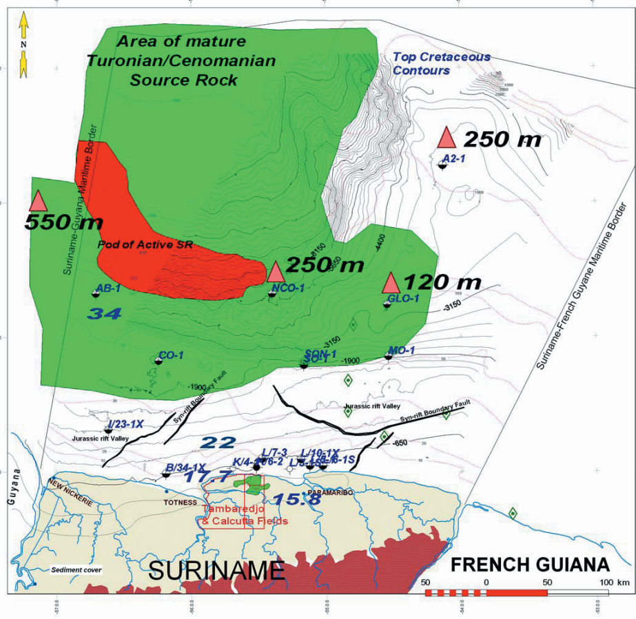
Figure 17: Cenomanian-Turonian Source Rock
