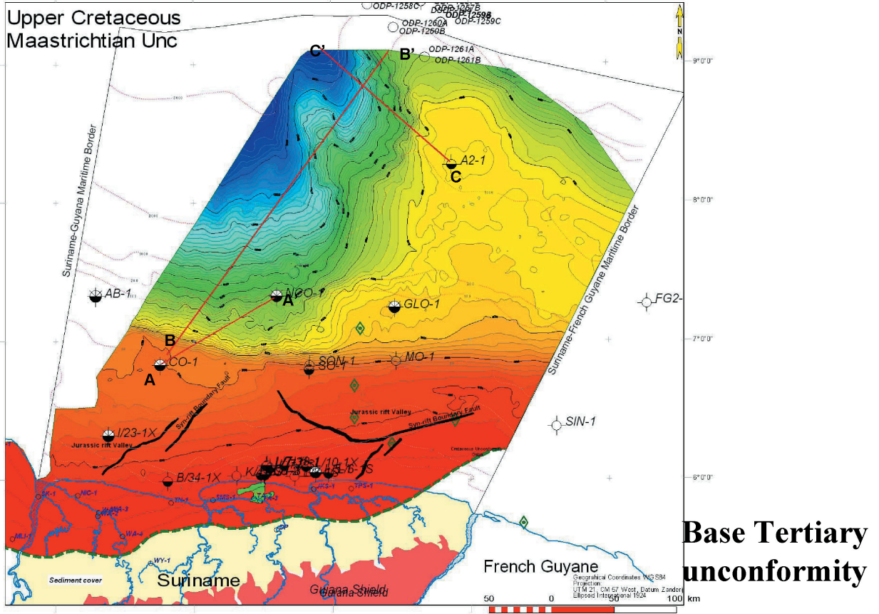
Figure 10: Upper Cretaceous, Maastrichtian unc. map
