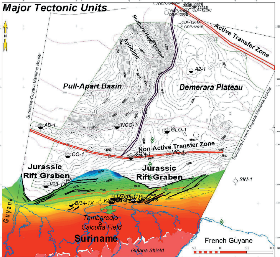
Figure 8: Major tectonic elements in the Suriname-Guyana Basin
